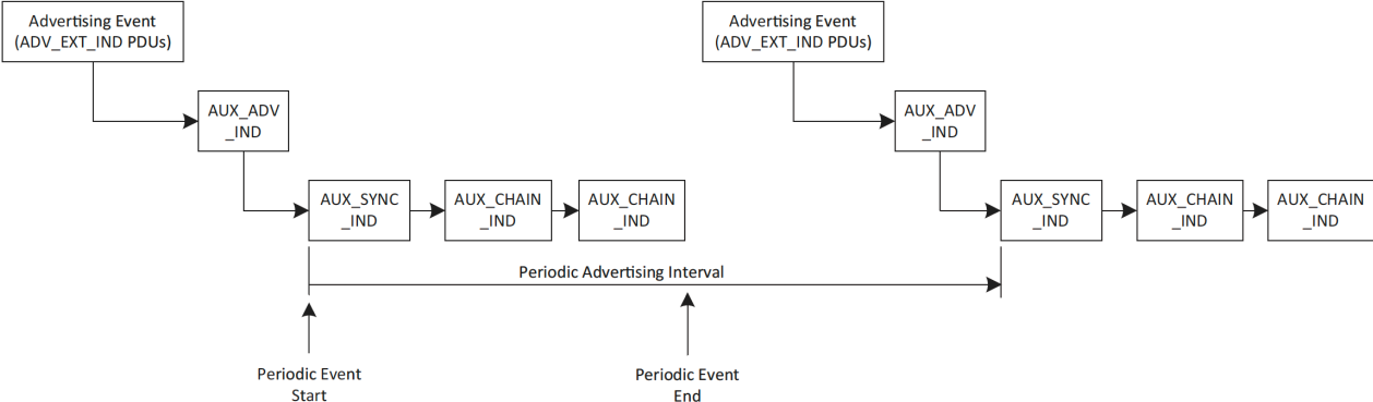
Figure 21: Periodic advertising (Source: Bluetooth 5 specification document)
